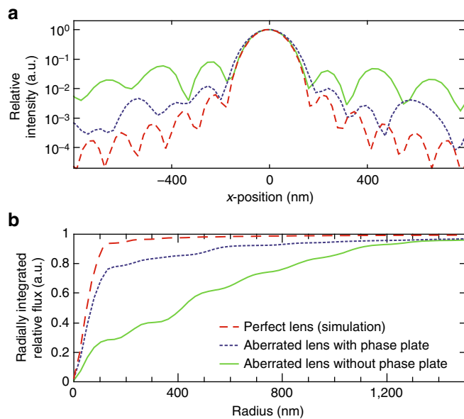
Figure 4 | Improved focal spot characteristics. (a) Horizontal slice (x-direction, logarithmic scale) through the focal plane depicted in Fig. 3b,e and for an ideal lens. (b) Radially integrated intensity distribution around the centre of the focal spot. The solid green line represents the results for the uncorrected lens (without the phase plate), the dotted blue line represents the phase plate corrected lens, and the dashed red line represents the modelled aberration-free lens in both a,b .
