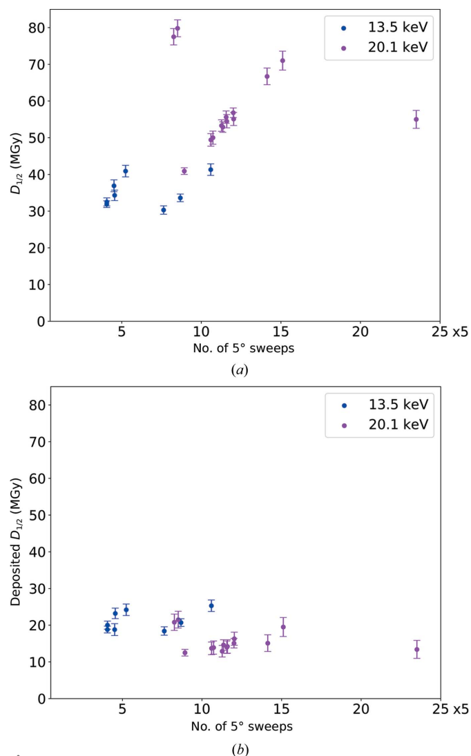
Figure 3 (a) D_{1/2} values for 22 crystals with an average size of 5.2 \times 3.1 \times 3.1 \mu\text{m} with a beam size of 6.4 \times 7.2 \mu\text{m} collected from the same grid at 13.5 keV (blue) and at 20.1 keV (magenta) plotted with error bars representing measurement errors in flux, crystal size and fit of the decay curve. (b) As in (a) but plotted against the dose corrected for photoelectron escape, referred to as the deposited dose.
