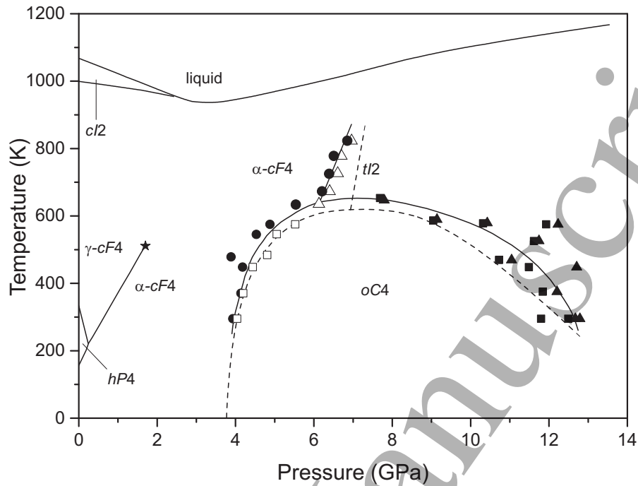
Figure 4. The proposed P-T phase diagram of Ce. The data were collected along a series of isotherms, and the filled circles mark the highest pressure at which single-phase \alpha -cF4 diffraction patterns were observed at each temperature, while the unfilled squares and triangles immediately to their right show the pressures at which the oC4 and tI2 phases, respectively, were first observed on compressing the same samples. Similarly, at higher pressures, the filled squares mark the highest pressure at which single-phase oC4 diffraction patterns were observed, while the filled triangles to their right show the pressures at which the tI2 phase was first observed in the same samples. The dashed lines show the phase boundaries reported by Schiwek et al. [6], and references therein, while the solid lines show the phase boundaries that best-fit the current data.
