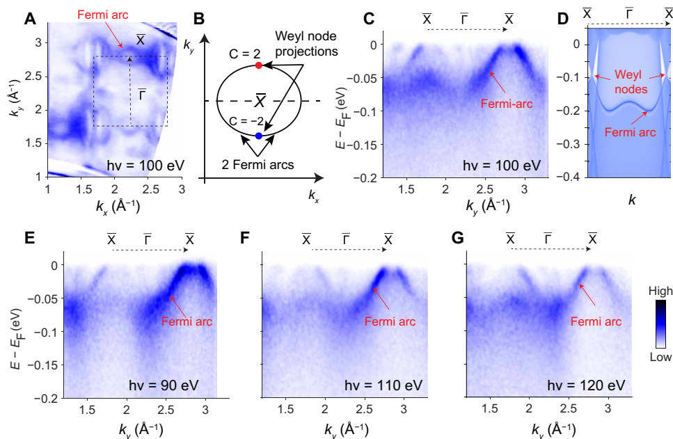
Fig. 4. Surface state structure on the (100) surface. (A) Experimental Fermi surface measured on the (100) cleavage plane with photon energy h\nu = 100 eV and linear-horizontal polarization. The dashed black line indicates the boundary of the surface Brillouin zone, and the black dashed arrow indicates the momentum direction of the line cuts shown in (C) to (F). (B) Illustration of the Fermi arcs and Weyl point projections in the vicinity of the surface Brillouin zone boundary (black dashed line) at the \bar{X} point. Red and blue dots indicate Weyl point projections, and black arrows indicate Fermi arc positions. (C) Experimental band dispersion of the Fermi arc surface states along the line cut shown in (A). The photon energy used here was h\nu = 100 eV and the polarization was linear-horizontal. (D) Calculated surface state dispersion along the same momentum direction as the experimental line cuts. (E to G) Same as in (B) but for photon energies of 90, 110, and 120 eV.
