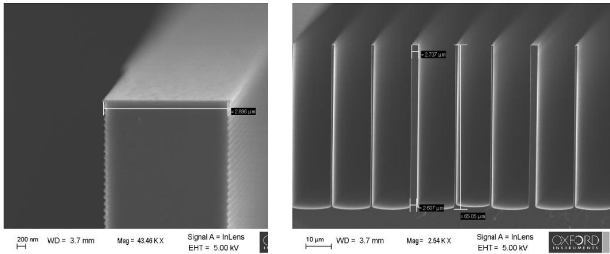
Figure 2. SEM image of a 65 \mu\text{m} thick test structures etched with the planar silicon kinoform lenses in the etch optimisation process. Scalloping < 50 nm and etch angle \theta = 89.9^\circ .
