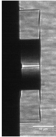
Figure 3. X-ray topographic images of a kinoform lens with focal length f = 30 mm, acquired on highly coherent synchrotron beamline I13-1 at Diamond Light Source. The lens is aligned to provide vertical focusing. The bright line at the centre is the focused radiation. The dark area on the left is the supporting wafer; the dark area around the focal line is the shadow of the lens body. Refraction from borders of a pre-collimating large radius elliptical surface, visible in the SEM in Figure 1 can be observed.
