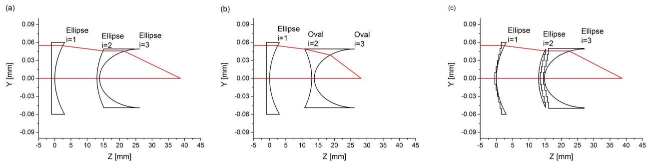
Figure 5. Schematic representation of aberration-free x-ray lens designs composed of (a) elliptical refractive surfaces, (b) ellipses and Ovals of Descartes and (c) compound elliptical kinoform structures [3]. The principal rays are shown in red. All geometrical rays refracted through the single elements are parallel to the kinoform steps. This is a necessary condition for phase preservation of the x-ray beam in the lens material.
