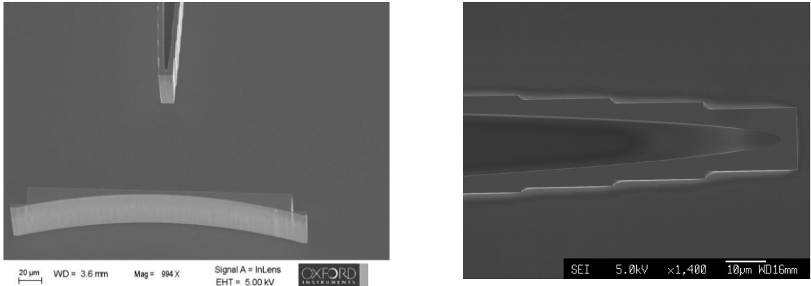
Figure 1. SEM images of planar silicon kinoform lens detail, with a radius at the apex of R = 150 nm
