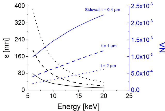
Figure 4. Diffraction limit s for silicon kinoform lenses (black curves) and numerical aperture NA (blue curves). The solid curves are calculated for t = 0.4 \mu\text{m} , the dashed lines for t = 1 \mu\text{m} and the dotted lines for t = 2 \mu\text{m} .
